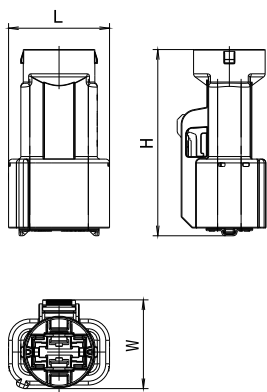
Receptacle Housing 180°
