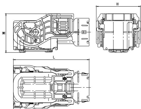
Receptacle Housing 90°
