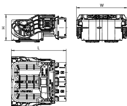
Receptacle Housing 90°
